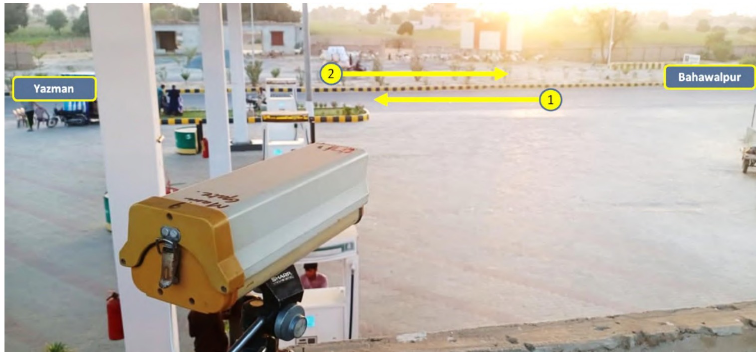
Figure 7 - Camera location at site (MB-1)
